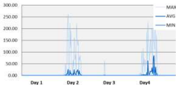
Snowdrift (g/m 2 /s)
